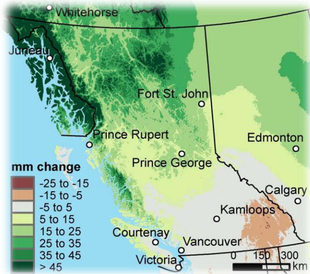
B.C. summer precipitation change expected in the 2050s based on 1961-1990 baseline precipitation. Courtesy: Climate Impacts Consortium
